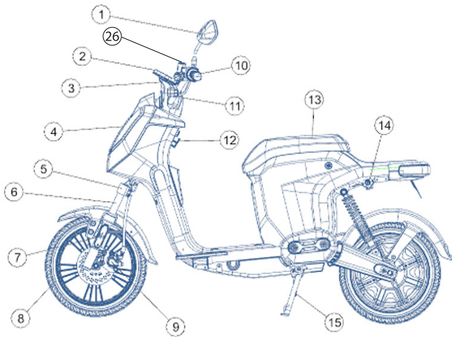
Fig. 1 Side view of the vehicle
