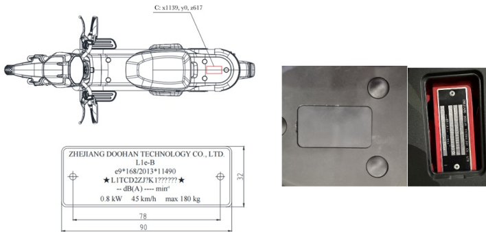
Fig. 5 Information label
